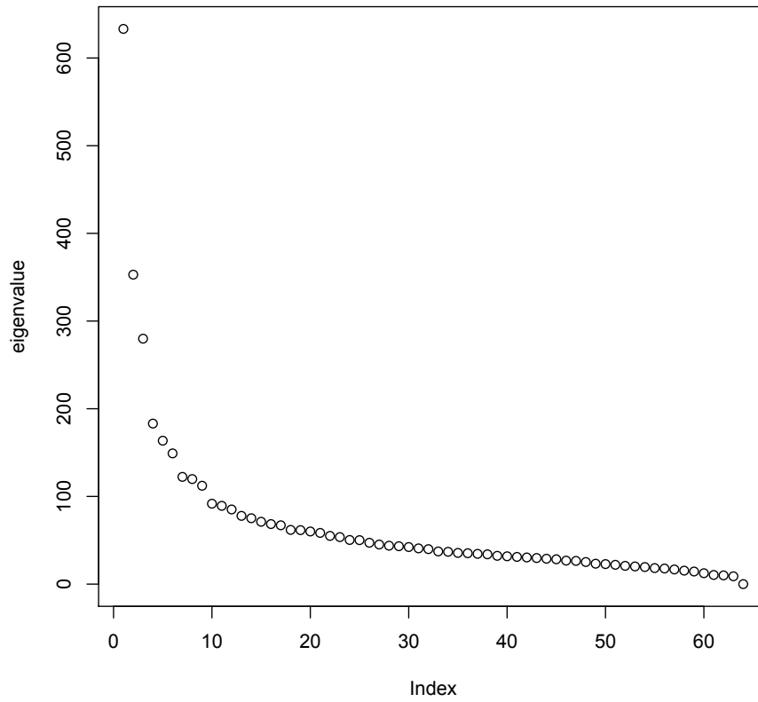
Scree plot for Homework 4
