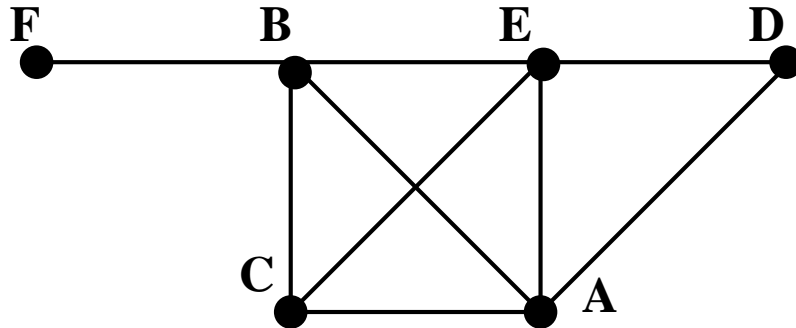
Fig. 1. Independence graph induced by the marginals [BF], [ABCE] and [ADE]
