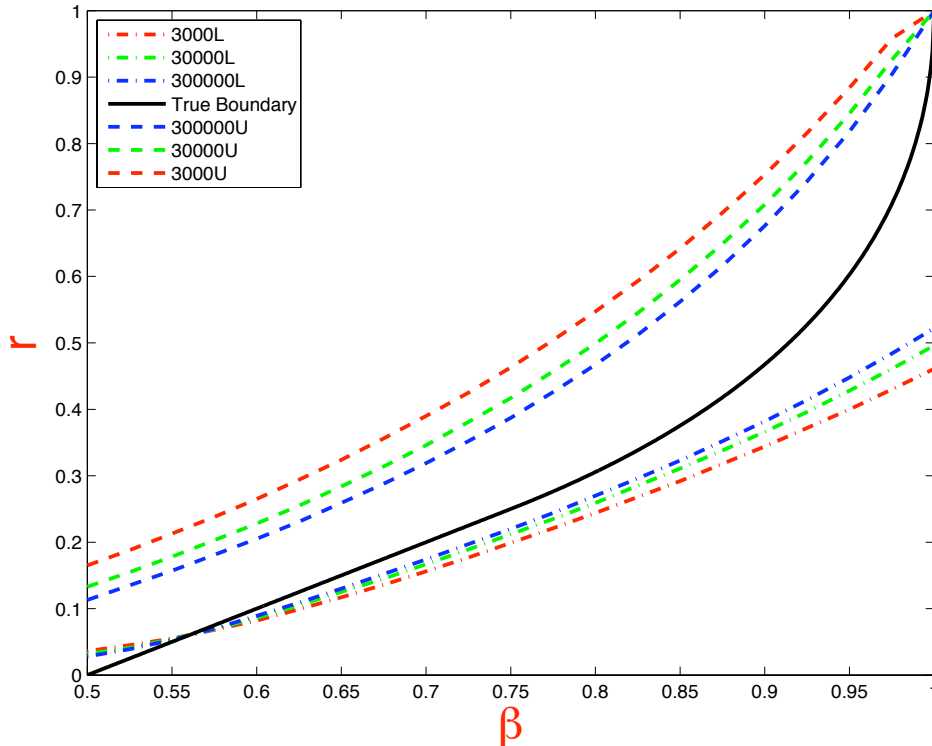
Figure 4: Classification boundaries for p = 3 \times 10^3 \times (1, 10, 100) . For each p , both an upper boundary and a lower boundary are calculated which correspond to the proxy classification errors of 10% and 40% using ideal HCT. The gap between two boundaries gets smaller as p increases. The solid black curve displays the asymptotic boundary r = \rho^*(\beta) .
