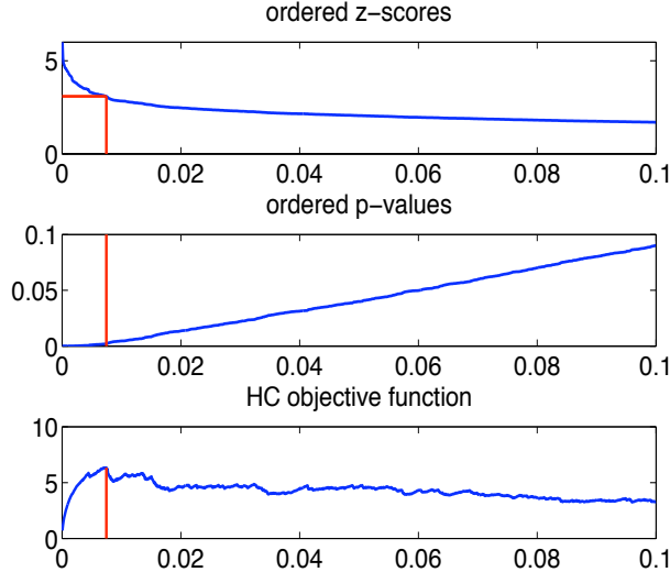
Figure 1: Illustration of HC thresholding. Panel (a) the ordered |Z| -scores. Panel (b) the corresponding ordered P -values in a PP plot. Panel (c) the HC objective function in (1.1); this is largest at i \approx 0.007p ( x -axes are i/p ). Vertical lines indicate \pi_{(i)} in Panel (b), and |Z|_{(i)} in Panel (a).
