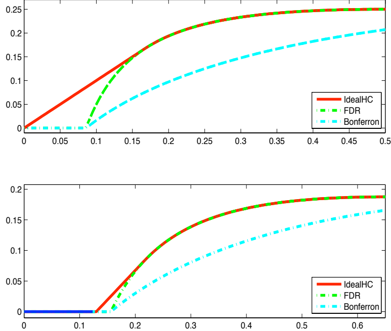
Figure 3: Comparison of SEP exponents for HCT, FDRT, and Bonferroni. Top: \beta = 1/2 . Bottom: \beta = 5/8 . x -axes displays r -values from 0 to \beta , y -axes display corresponding exponents. Solid blue horizontal bar indicates that r falls in the failure region where all exponents are 0.
