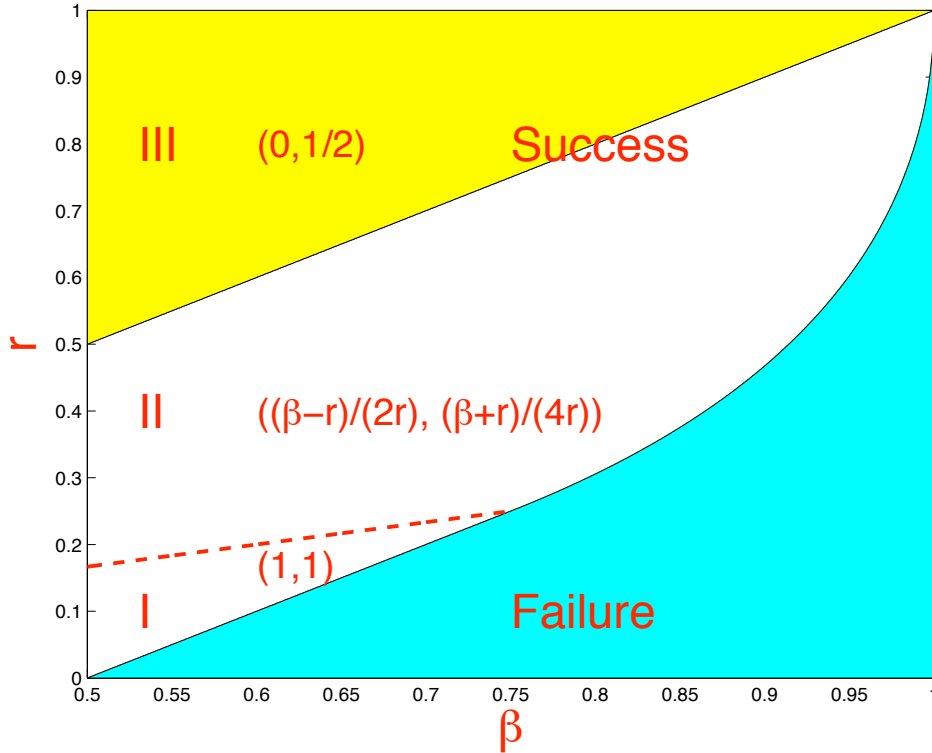
Figure 2: Phase diagram. The curve r = \rho^*(\beta) splits the phase space into the failure region and the success region, and the latter further splits into three different regions I, II, III. Numbers in the brackets show limits of \widehat{FDR} and \widehat{Lfd} at the ideal HCT as in Theorem 4.
