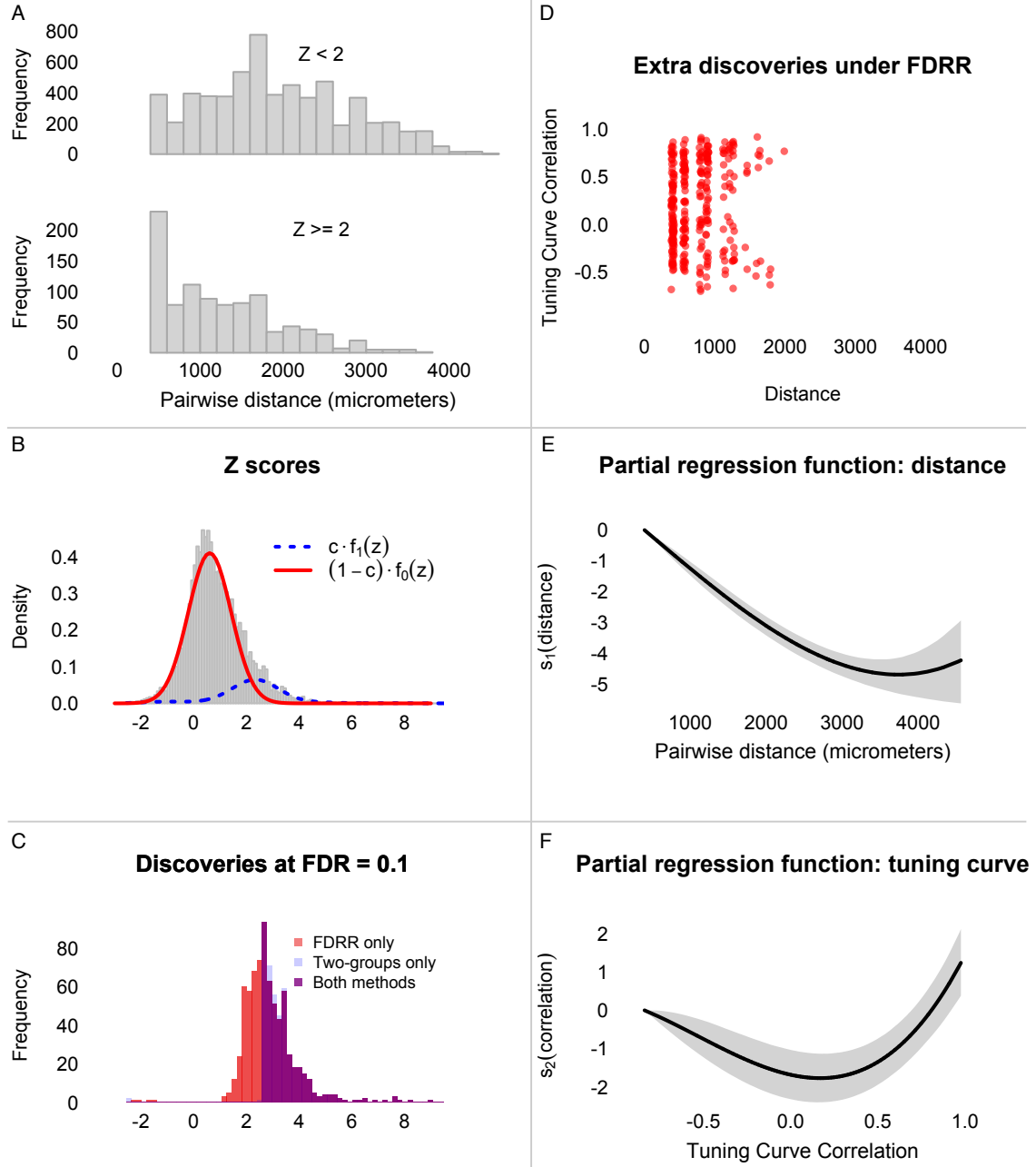
Figure 3: Panel A shows histograms of inter-neuron distances for pairs with synchrony z -score less than 2, versus those with z -score larger than 2. Panel B shows the empirical null density f_0(z) , together with the signal density f_1(z) estimated by predictive recursion, superimposed upon the histogram of the raw z -scores. Panel C compares discoveries at the 10% FDR level using the ordinary two-groups local FDR model, versus those under the FDR regression model. Panel D shows that the extra discoveries made by FDR regression (red points) tend to concentrate at short inter-neuron distances compared with the rest of the neuron pairs. Panels E and F show the estimated partial regression functions for prior log-odds of being a signal versus distance and tuning curve correlation. The black lines are the estimates, and the grey areas show 95% posterior credible intervals arising from the full Bayes analysis.
