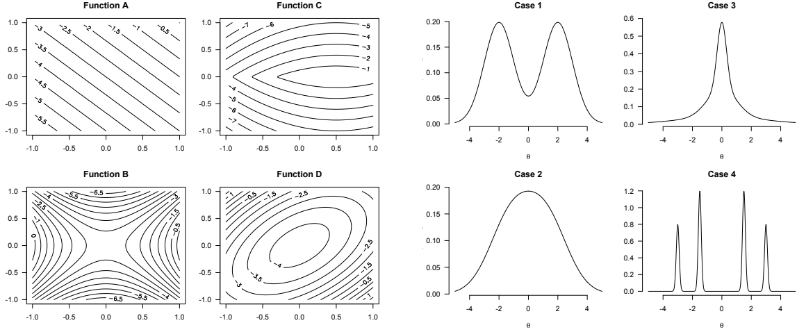
Figure 1: Settings for the simulation study. Left four panels: choices for the bivariate regression function s(x_1, x_2) . The contours show the prior log odds that a test statistic in that part of covariate space will be a signal. Function E, not shown, is a flat function: s(x) = -3 . Right four panels: choices for \pi(\theta) .
