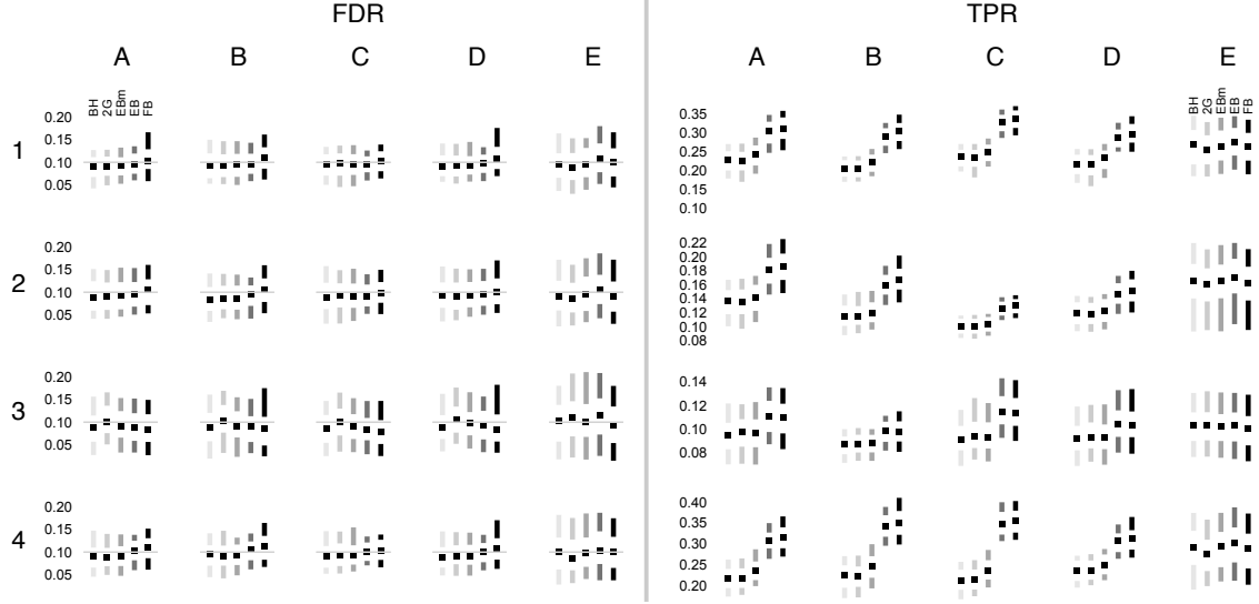
Figure 2: Boxplots of false discovery rate (FDR, left 20 panels) and true positive rate (TPR, right 20 panels) for the simulation study. The rows are the different true priors \pi(\theta) , and the columns are the different true regression function s(x_1, x_2) . Within each panel, the boxplots show the median, interquartile range (white bar), and range (grey bar) for each method across the 100 simulated data sets. Within each panel, the methods are arranged from left to right as: Benjamini–Hochberg (BH), the two-groups model without covariates (2G), empirical Bayes with marginalization (EBm, Section 2.2), empirical Bayes (EB, Section 2.1), and fully Bayes (FB, Section 2.3).
