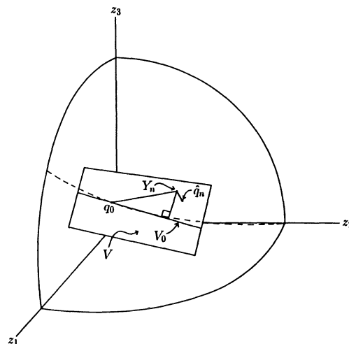
FIG. 2. The subspace V_0 of the tangent plane V at q_0 . Y_n is the image of \hat{q}_n under the mapping F defined by (2.18).
