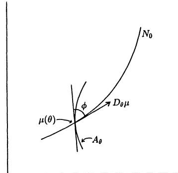
FIG. 6. The angle between N_0 and A_\theta is the angle \phi .
