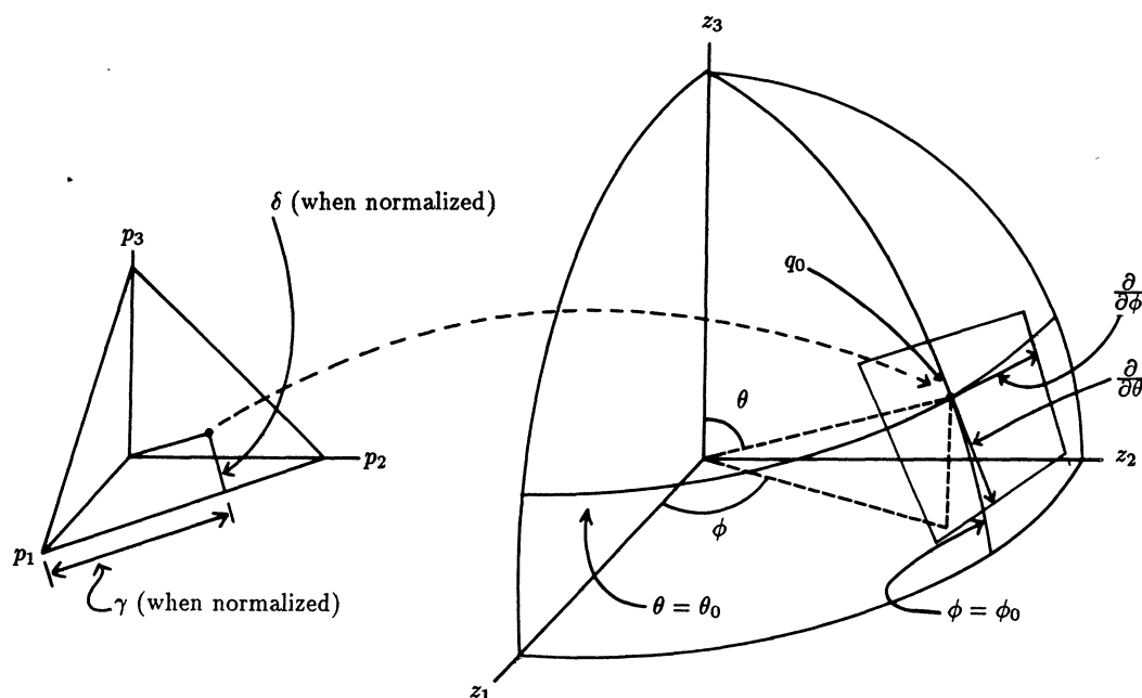
FIG. 1. The transformation from (p_1, p_2, p_3) -space to (z_1, z_2, z_3) -space, with polar coordinates \theta = \arccos(p_3^{1/2}) , \phi = \arcsin((p_2/(p_2 + p_3))^{1/2}) . The vectors \partial/\partial\theta and \partial/\partial\phi are tangent to the coordinate curves defined by the polar coordinates (\theta, \phi) .
