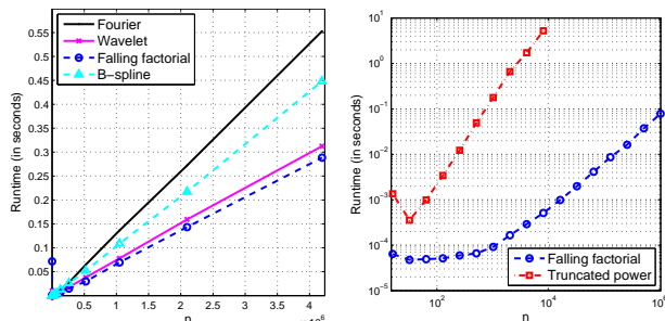
(a) Falling factorial vs. Fourier, wavelet, and B-spline transforms (linear scale) (b) Falling factorial (H) vs. truncated power (G) transforms (log-log scale)
