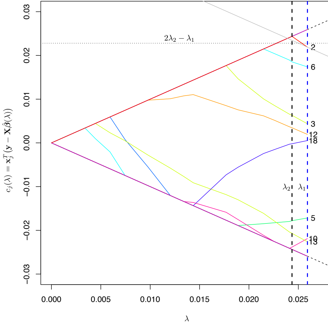
Fig. 5. Example of a violation of the slope bound (10), which breaks the sequential strong rule (6). The entries of y and X were generated as independent, standard normal random variables with N = 50 and p = 30 . (Hence there is no underlying signal.) The lines with slopes \pm\lambda are the envelopes of maximal inner products achieved by predictors in the model for each \lambda . For clarity we only show a short stretch of the solution path. The blue dashed vertical line is drawn at \lambda_1 , and we are considering the the solution at a new value \lambda_2 < \lambda_1 , the black dashed vertical line to its left. The dotted horizontal line is the bound (6). In the top right part of the plot, the inner product path for the predictor j = 2 is drawn in red, and starts below the bound, but enters the model at \lambda_2 . The slope of the red segment between \lambda_1 and \lambda_2 is -1.586 . A gray line of slope -1 is drawn beside the red segment for reference. The plot contains other examples of large slopes leading to rule violations, for example, around \lambda = 0.007 .
