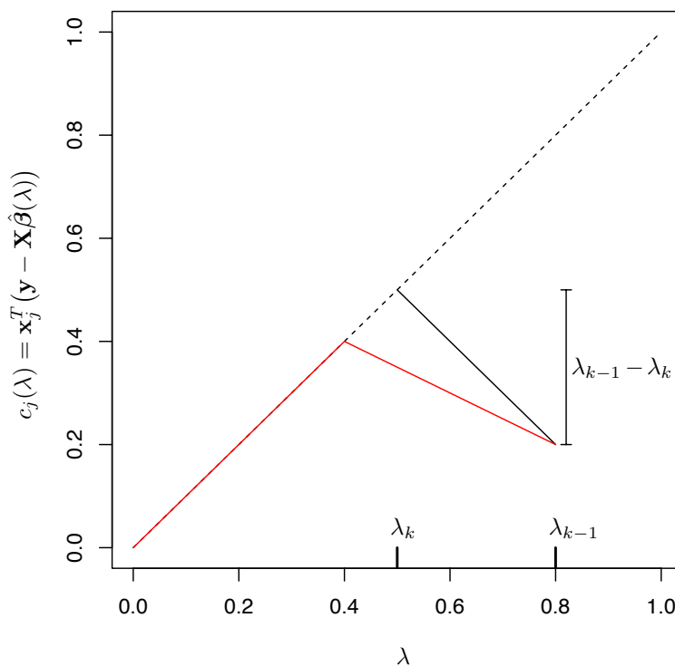
Fig. 4. Illustration of the slope bound (10) leading to the strong rules (5) and (6). The inner product c_j is plotted in red as a function of \lambda , restricted to only one predictor for simplicity. The slope of c_j between \lambda_{k-1} and \lambda_k is bounded in absolute value by 1 (black line), so the most it can rise over this interval is \lambda_{k-1} - \lambda_k . Therefore, if it starts below \lambda_k - (\lambda_{k-1} - \lambda_k) = 2\lambda_k - \lambda_{k-1} , it cannot possibly reach the critical level by \lambda_k .
