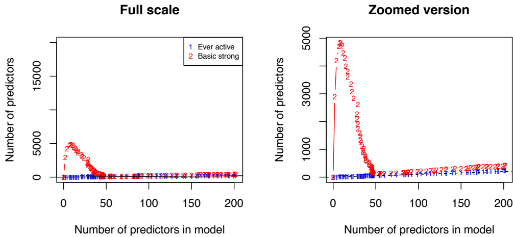
Fig. 10. Gaussian lasso setting, N = 200 , p = 20,000 , pairwise correlation between features of 0.7. The first 50 predictors have positive, decreasing coefficients. Shown are the number of predictors left after applying the strong sequential rule (6) and the number that have ever been active (that is, had a nonzero coefficient in the solution) for values of \lambda larger than the current value. A broken line with unit slope is added for reference. The right-hand plot is a zoomed version of the left plot.
