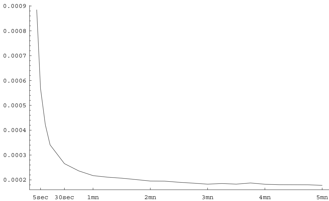
Figure 1: This figure shows the RV estimator [Y, Y]_T^{(\text{all})} plotted against the sampling interval \Delta . Since \Delta = T/n , the plot illustrates the divergence of RV as n \rightarrow \infty predicted by our theory: RV has bias 2nE[\varepsilon^2] .
