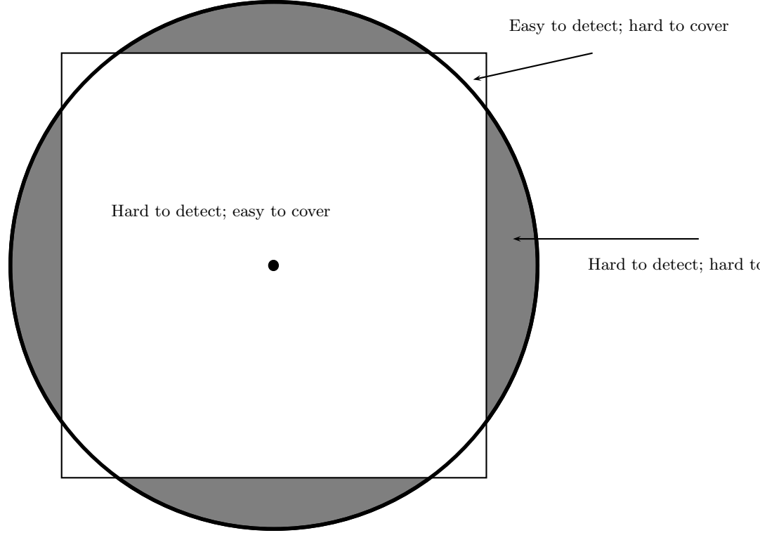
FIG 3. The dot at the center represents the subspace \mathcal{F} . The shaded area is the set of spoilers \mathcal{S}(\epsilon_2, \epsilon_\infty) of vectors for which f^* \neq f . If these vectors were not surrogated, adaptation is not possible. The non-shaded area is the invariant set \mathcal{I}(\epsilon_2, \epsilon_\infty) = \{f : f^* = f\} .
