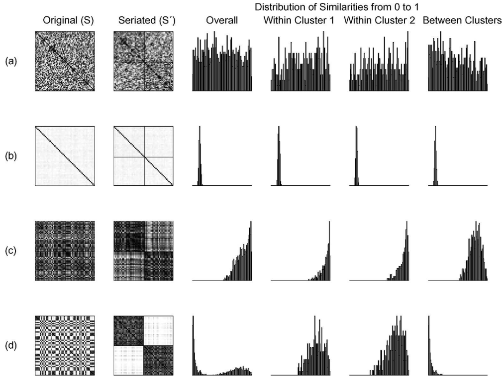
Figure 2 Illustrative Clusion Patterns in Original Order and Seriated Using Optimal Bipartitioning Are Shown in the Left Two Columns. The Right Four Columns Show Corresponding Similarity Distributions. In Each Example There Are 50 Objects: (a) No Natural Clusters (Randomly Related Objects), (b) Set of Singletons (Pairwise Near Orthogonal Objects), (c) One Natural Cluster (Unimodal Gaussian), (d) Two Natural Clusters (Mixture of Two Gaussians)
