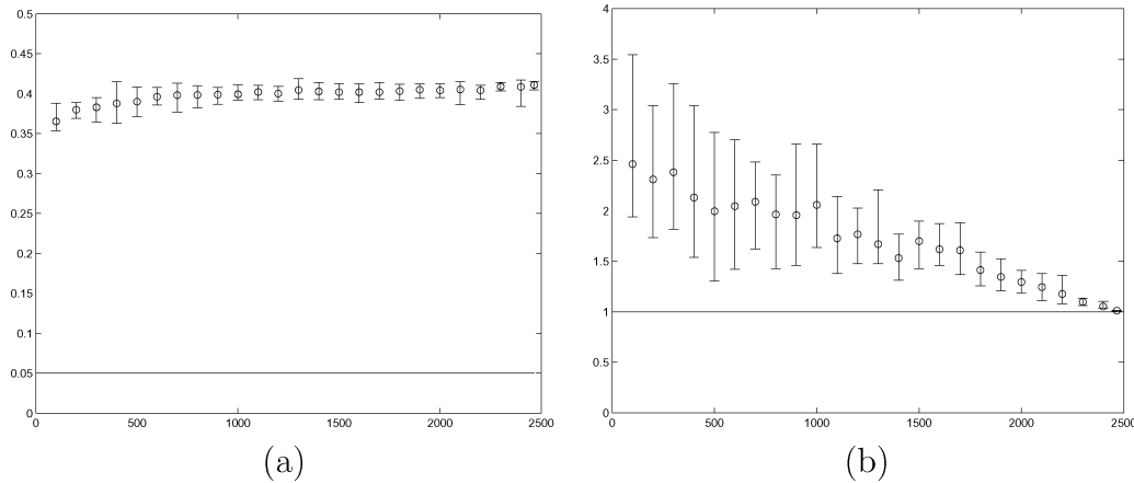
Figure 7 Effect of Sub-Sampling on OPOSSUM. Cluster Quality As Measured by Remaining Edge-Weight Fraction (a) and Imbalance (b) of Total Graph With 2466 Vertices (customers from Section 5.1) for Various Boot Sample Sizes n in FASTOPOSSUM. For Each Setting of n the Results' Range and Mean of 10 Trials Are Depicted
