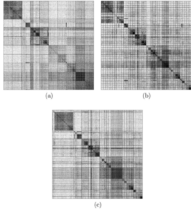
Figure 5 Comparison of Various Number of Clusters k for Yahoo! News Data: (a) Under-Clustering at k = 10 , (b) Over-Clustering at k = 40 , (c) Good Clustering Through Interactive Split and Merge Using CLUSION at k = 20
