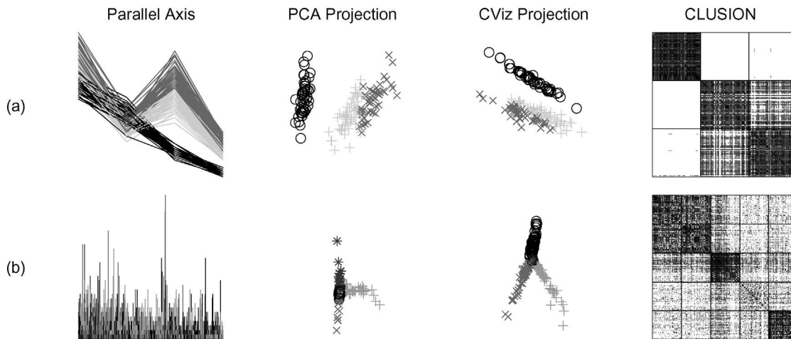
Figure 3 Comparison of Cluster-Visualization Techniques. All Tools Work Well on the Four-Dimensional IRIS Data (a). But on the 2903-Dimensional Yahoo! News-Document Data (b), Only CLUSION Reveals that Clusters 1 and 2 Are Actually Highly Related, Cluster 3 Is Strong and Interdisciplinary, 4 Is Weak, and 5 Is Strong
