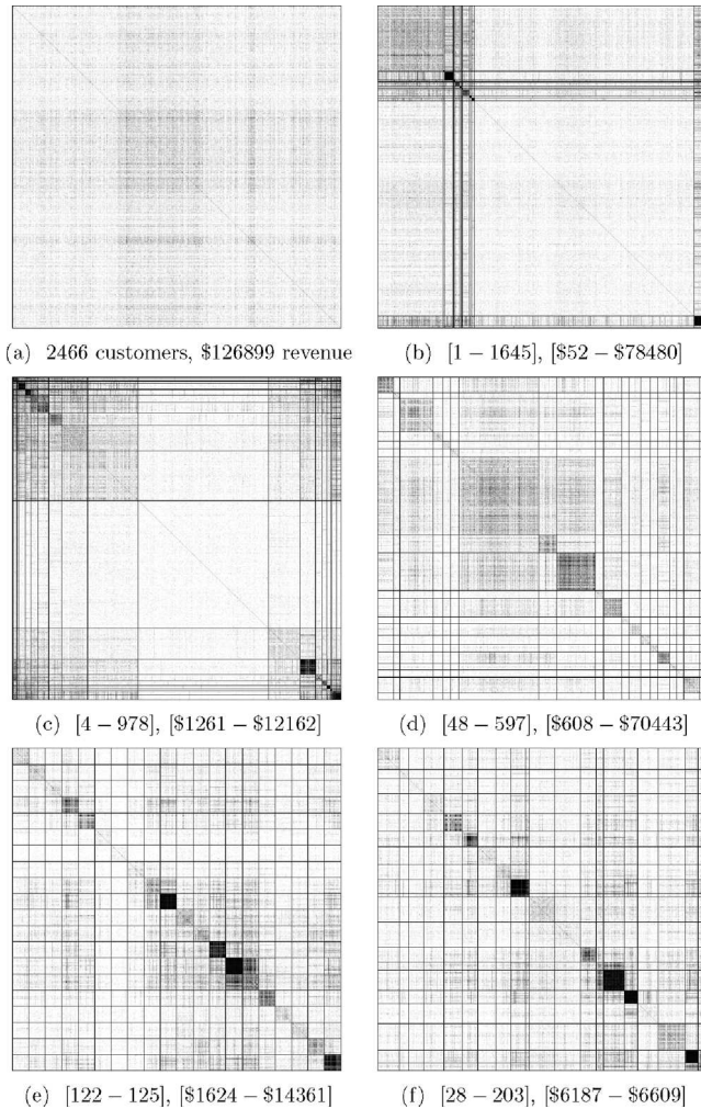
Figure 4 Visualizing Partitioning Drugstore Customers into 20 Clusters. Relationship Visualizations Using CLUSION: (a) Original (Randomly) Ordered Similarity Matrix, (b) Partially Reordered Using Euclidean k -means, (c) Using SOM, (d) Using Standard Jaccard k -means, (e) Using Extended Jaccard Sample Balanced Opossum, (f) Using Value Balanced Opossum Clustering. Customer and Revenue Ranges Are Given Below Each Image
