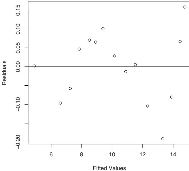
Fig. 5.4. Residual plot based on the model fit vapC0.m1 of the Antoine model fitted to the dataset vapC0 . A reference line with intercept 0 and slope 0 has been added using abline() .
