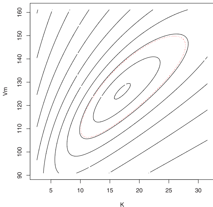
Fig. 2.4. Contour plot of the residual sums-of-squares function RSS(K, V_m) for the Michaelis-Menten model fitted to the dataset L.minor . The region encompassed by the dashed contour is a 95% confidence region (see Chapter 7 for more details).
