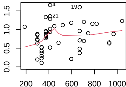
Scale-Location
