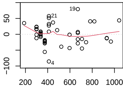
Residuals vs Fitted
