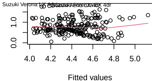
Scale-Location
