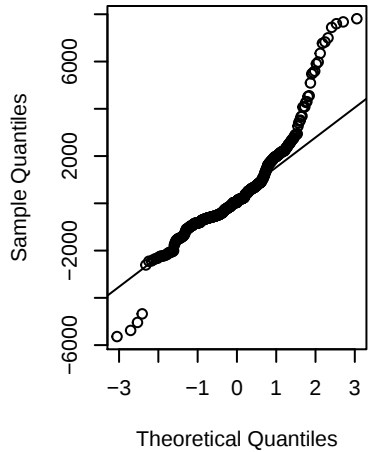
Random Residuals
