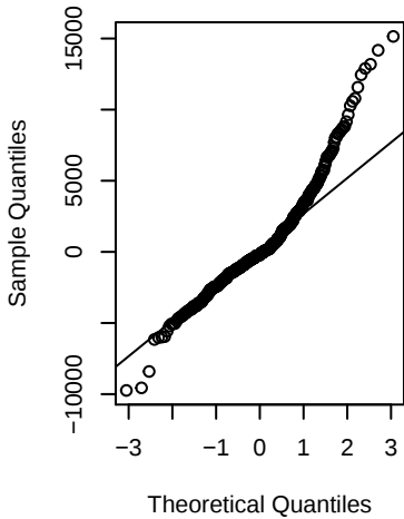
Marginal Residuals
