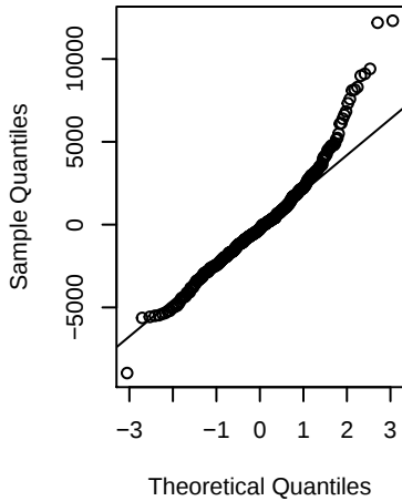
Conditional Residuals
