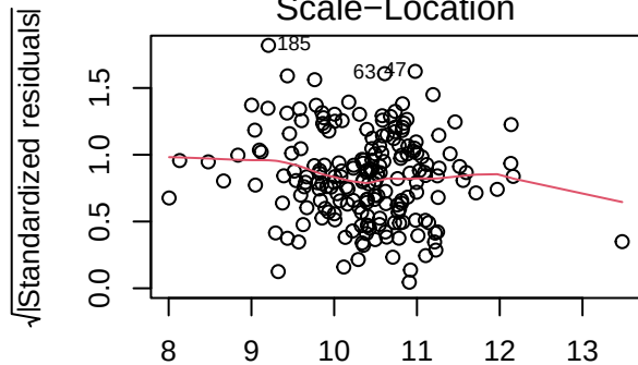
Scale-Location
