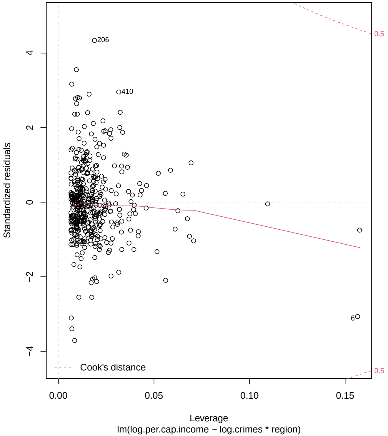
Residuals vs Leverage
