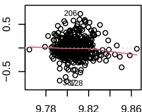
Residuals vs Fitted
