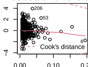
Residuals vs Leverage
