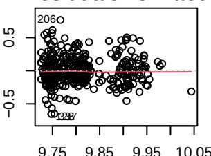
Residuals vs Fitted
