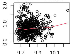
Scale-Location
