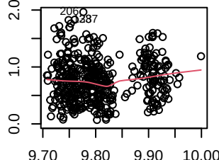
Scale-Location
