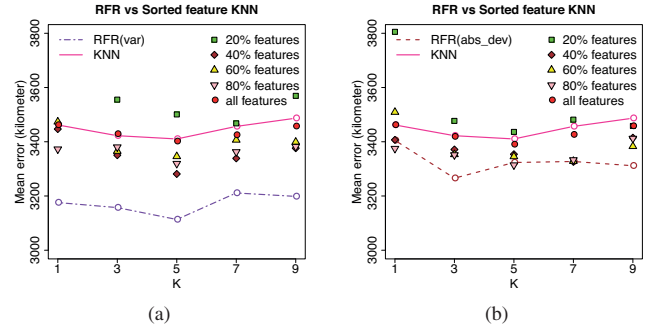
Fig. 5. Mean distance error as a function of K. The features are the default 68 features. The points are the results of KNN using a certain percentage of sorted features.
