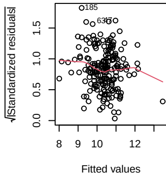
Scale-Location
