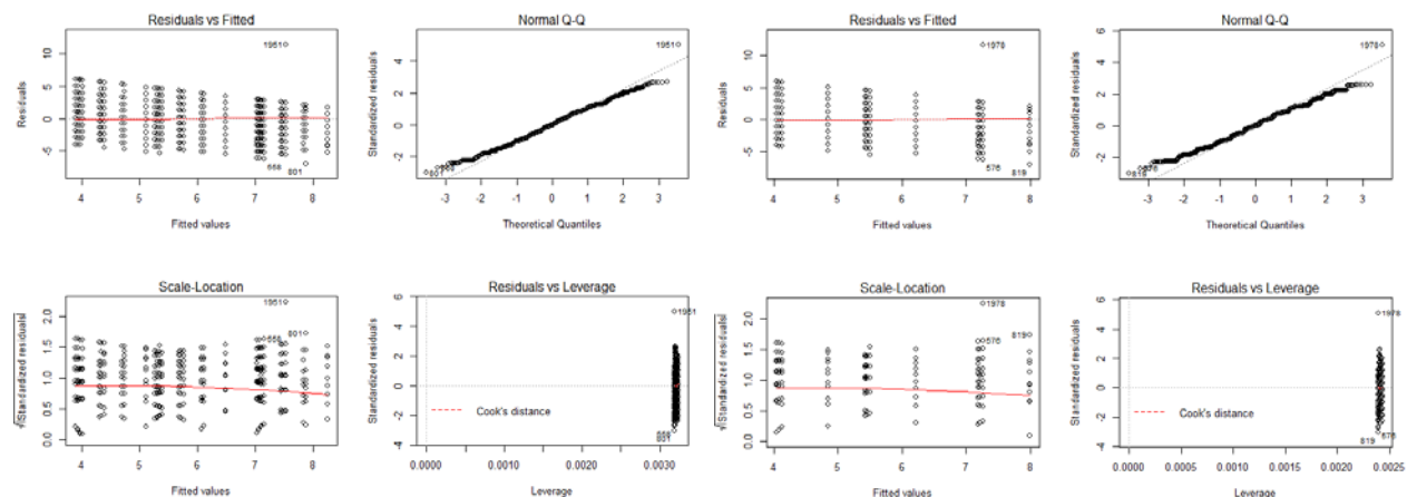
Figures: Diagnostic plots for fit.lm.full (left) and for fit.lm.3 (right)
