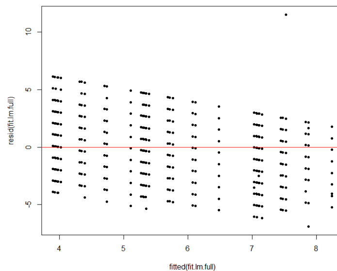
Figure: Residuals vs. fitted values for fit.lm.full
