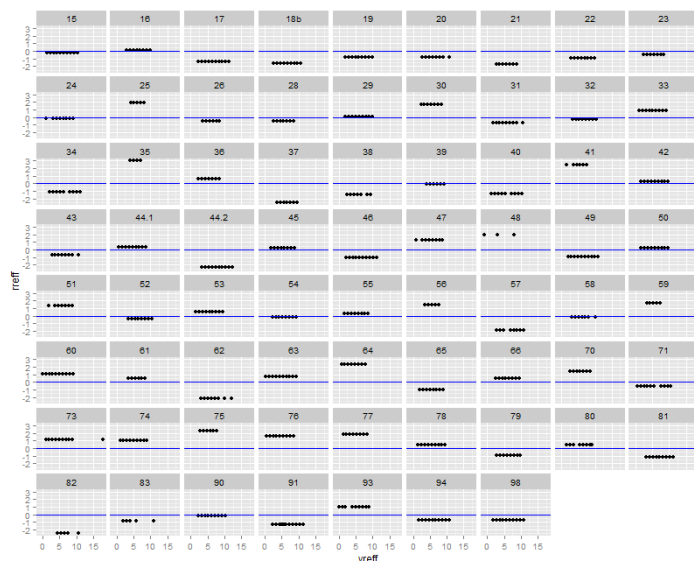
Figure: Marginal residuals vs. fitted (left, previous page), conditional residuals vs. fitted (right, previous page), and random effects residuals vs. fitted (left) for M1
