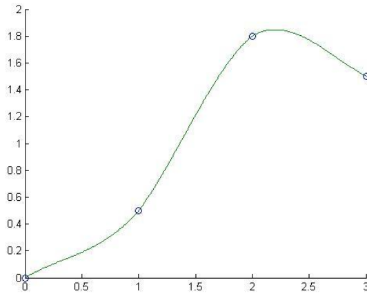
Figure 3. Clamped Cubic Spline.
