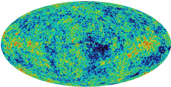
Image: NASA/WMAP Science Team
