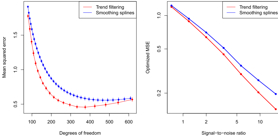
FIG. 4. The left panel shows the MSE curves for additive trend filtering (7) (of quadratic order) and additive smoothing splines (1) (of cubic order), computed over 10 repetitions from the heterogeneous smoothness simulation with n = 2500 and d = 10 , described in Section 5.1, where the SNR is set to 4. Vertical segments denote \pm 1 standard deviations. The right panel displays the best-case MSE for each method (the minimum MSE over its regularization path), in a problem setup with n = 1000 and d = 6 , as the signal-to-noise ratio (SNR) varies from 0.7 to 16, in equally spaced values on the log scale.
