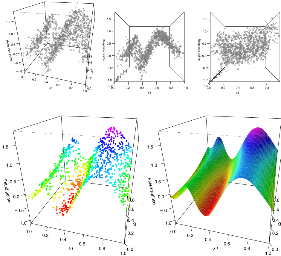
FIG. 3. An example of extrapolating the fitted additive trend filtering model, where n = 1000 and d = 2 . We generated input points X^i \stackrel{\text{i.i.d.}}{\sim} \text{Unif}[0, 1]^2 , i = 1, \dots, 1000 , and responses Y^i \stackrel{\text{i.i.d.}}{\sim} N(\sum_{j=1}^2 f_{0j}(X_j^i), \sigma^2) , i = 1, \dots, 1000 , where we f_{01}(x_1) = \sqrt{x_1} \sin(3\pi/(x_1 + 1/2)) and f_{02}(x_2) = x_2(x_2 - 1/3) , and \sigma = 0.36 . The top row shows three perspectives of the data. The bottom left panel shows the fitted values from additive trend filtering (7) (with k = 2 and \lambda = 0.004 ), where points are colored by their depth for visualization purposes. The bottom right panel shows the 2d surface associated with the trend filtering estimate, \hat{f}_1(x_1) + \hat{f}_2(x_2) over (x_1, x_2) \in [0, 1]^2 , with each component function extrapolated as in (13).
