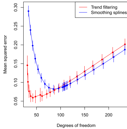
FIG. 2. MSE curves for additive trend filtering and additive smoothing splines, computed over 20 repetitions from the same simulation setup as in Figure 1. Vertical segments denote \pm 1 standard deviations. The MSE curves are parametrized by degrees of freedom (computed via standard Monte Carlo methods over the 20 repetitions).
