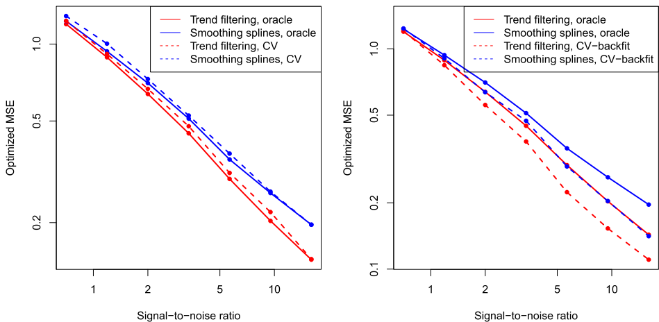
FIG. 5. Both panels display results from the same simulation setup as that in the right panel of Figure 4. The left panel shows MSE curves when the estimators are tuned by 5-fold cross-validation (CV), and also by the oracle (reflecting the minimum possible MSE). The right panel displays MSE curves when we allow each estimator to have d tuning parameters, tuned by a hybrid backfit-CV method explained in the text, versus the oracle MSE curves for a single tuning parameter.
